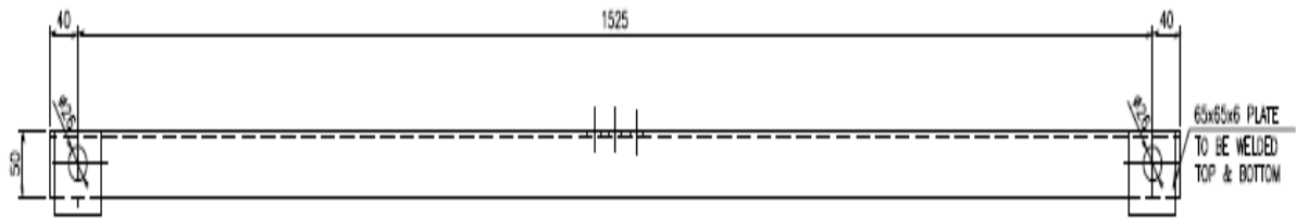
PLAN V-CROSS ARM(100x50x5)
