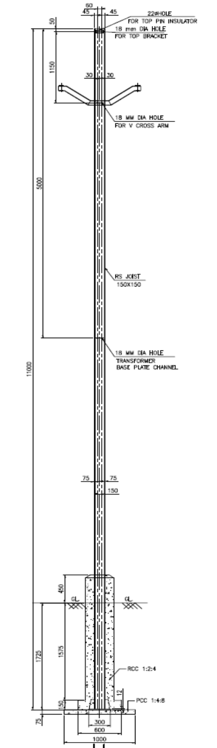
11KV LINE WITH RS JOIST 150X150 SINGLE POLE STRUCTURE
