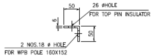
SECTION 1-1 (SCALE 1:5)
