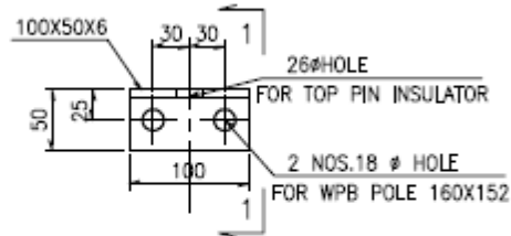
POLE TOP BRACKET (SCALE 1:5)
